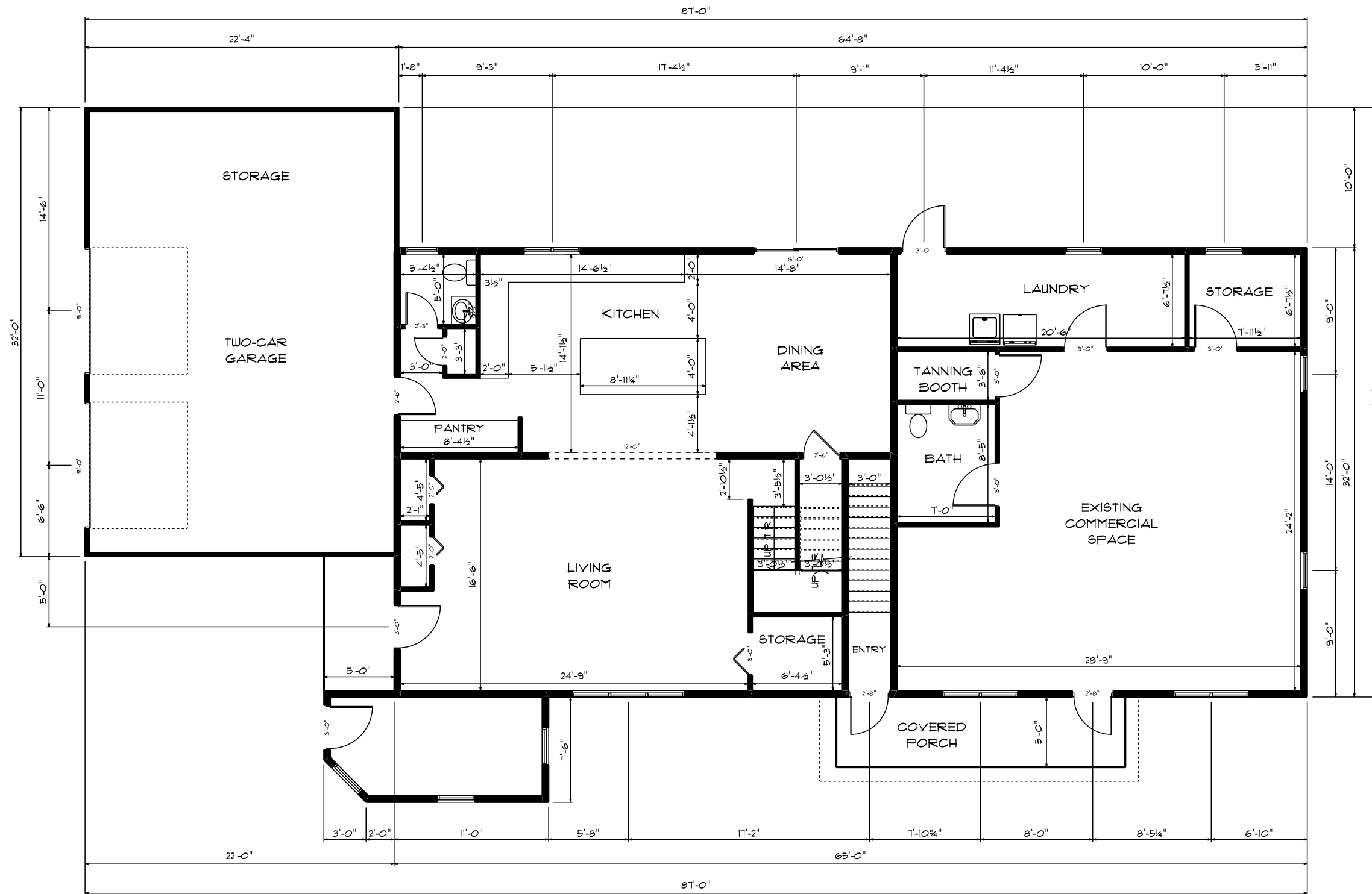
EXISTING FIRST FLOOR PLAN SCALE: 1/4" = 1'-0"
