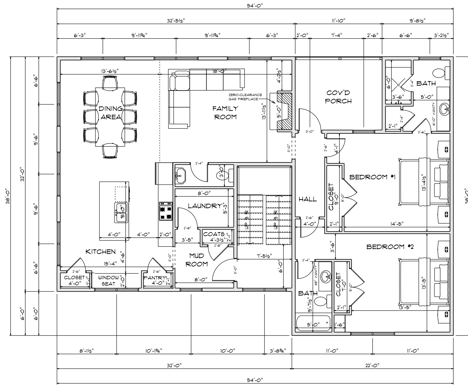
NORTH ADDITION - SECOND FLOOR PLAN SCALE: 1/4" = 1'-0"
