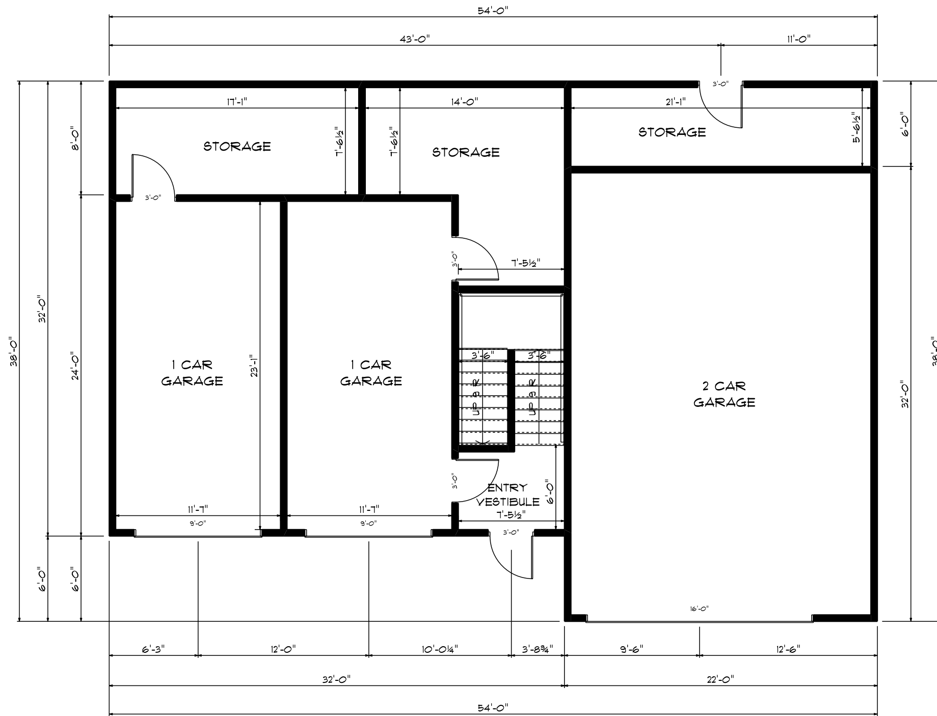
NORTH ADDITION - GARAGE PLAN SCALE: 1/4" = 1'-0"
