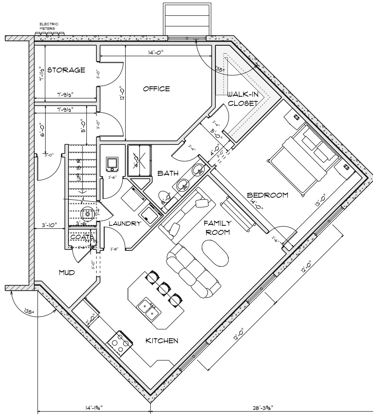
SOUTH BASEMENT SPACE SCALE: 1/4" = 1'-0"
