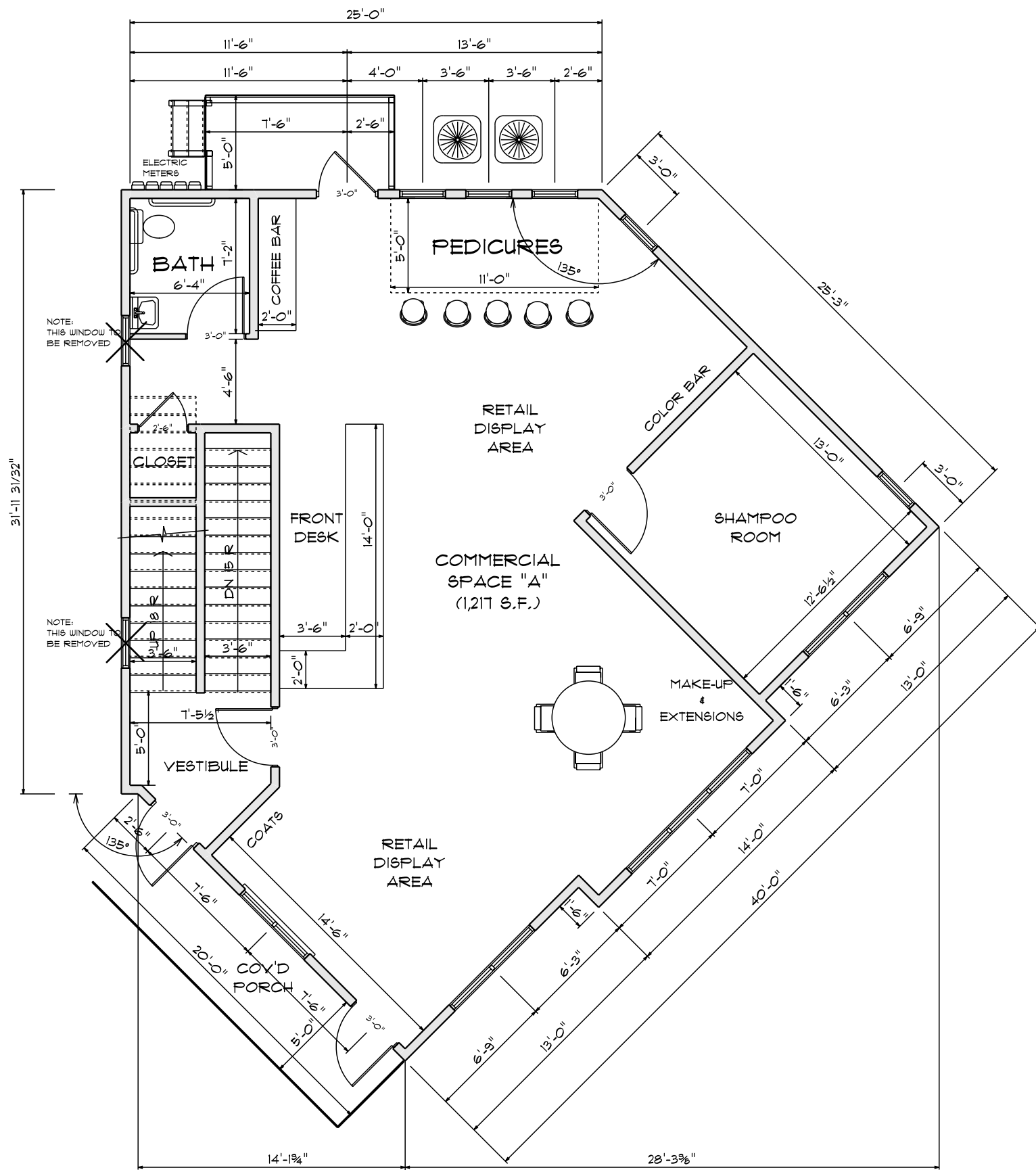
SOUTH ADDITION - FIRST FLOOR PLAN SCALE: 1/4" = 1'-0"
