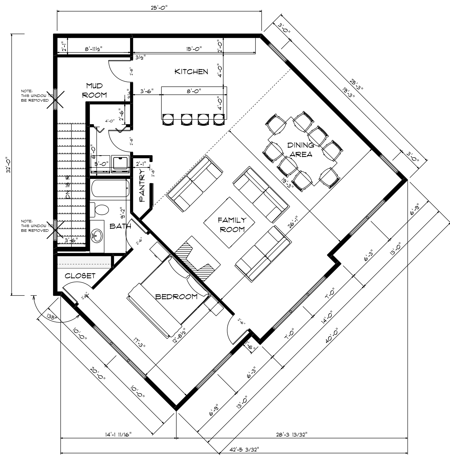
SOUTH ADDITION - SECOND FLOOR PLAN SCALE: 1/4" = 1'-0"
